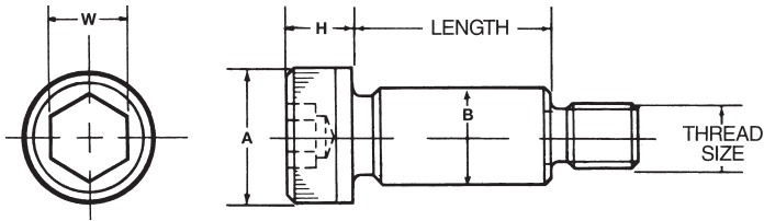
Dimensions to ISO 7379 Body Diameter to h8
