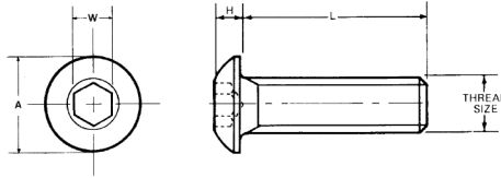
UNC/UNF Dimensions to ANSI B 18.3 BSW/BA Dimensions to BS 2470
