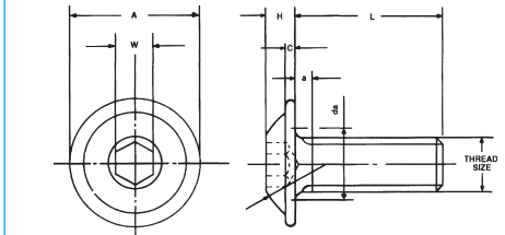
Dimensions to BS EN ISO 898/1 Grade 10.9 DIN 7380
