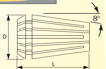
Collet Dimensions (mm)
