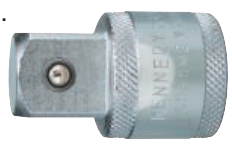
Male x male: 3/4" x 3/4".
